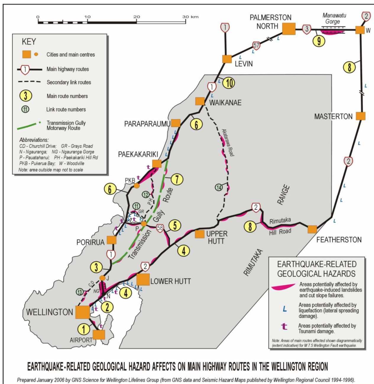
Figure 13: Earthquake-related geological hazard effects on the Wellington region's state highways. Source: Wellington Lifelines Group (2006).
