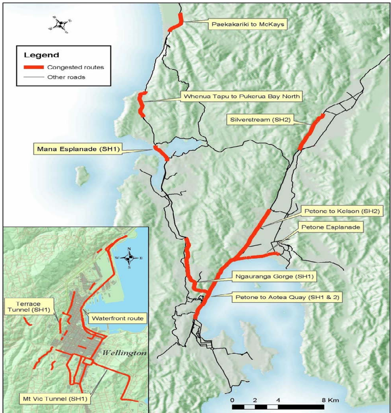
Figure 11: Wellington region's congestion bottlenecks. Source: Wellington Transport Strategic Model and other sources.
