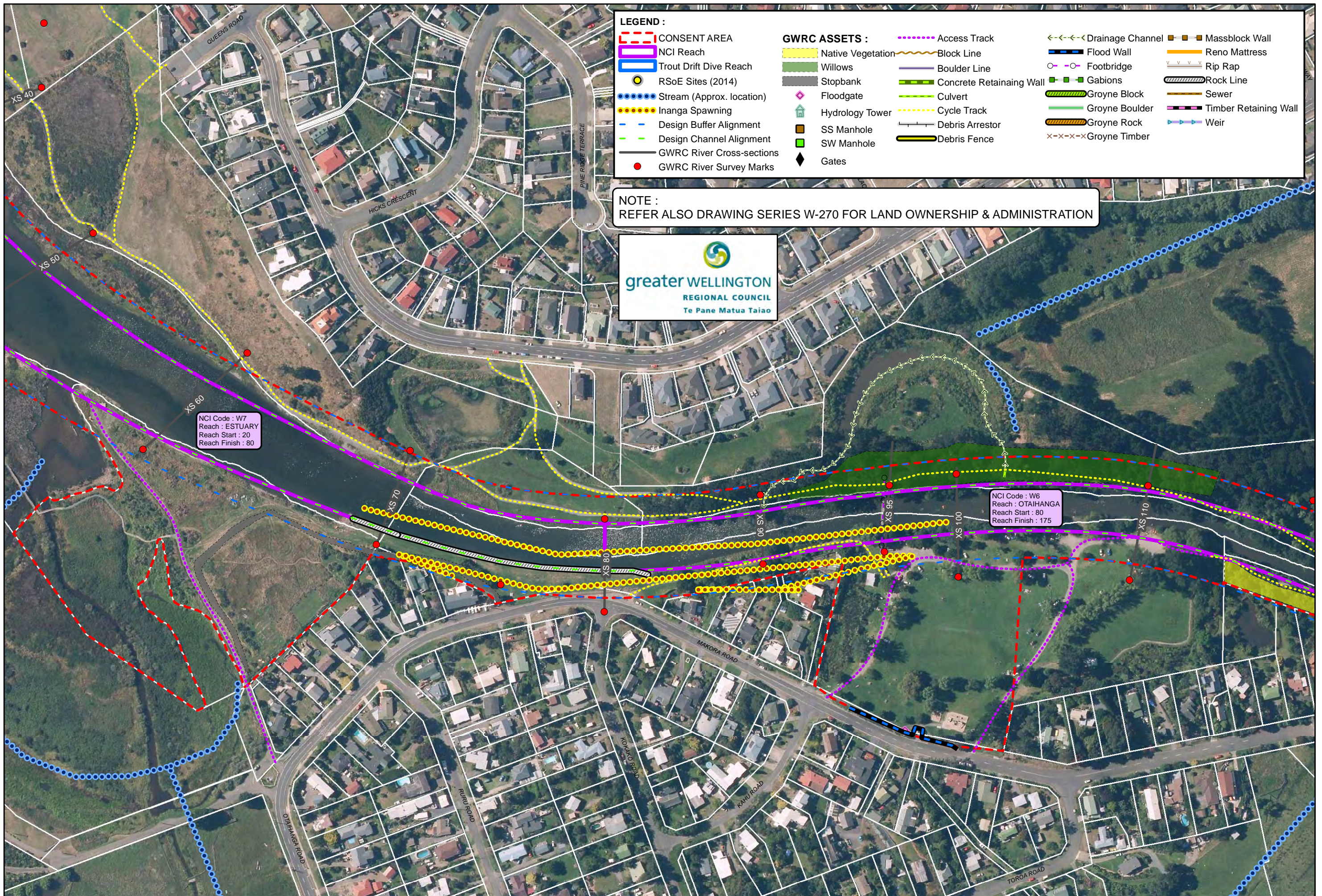
WAIKANAE RIVER - CONSENT AREA - Map 2a GWRC Asset, Fish & Ecological Information (River Mouth to Water Treatment Plant Weir)
