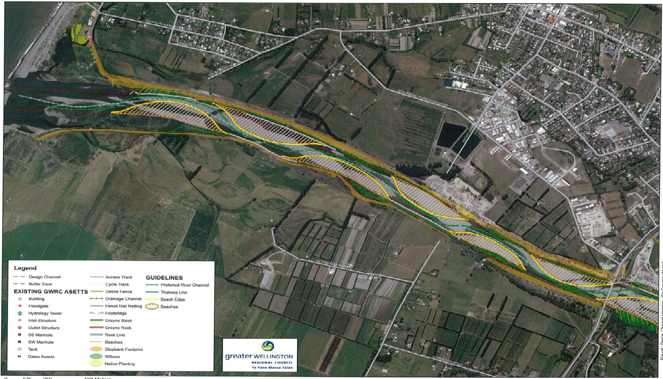
OTAKI RIVER - DESIGN CHANNEL MEANDER (Sheet 2 of 3)
