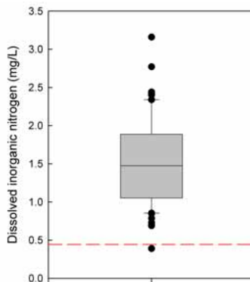
Figure 3.1: Box-and-whisker plot summarising dissolved inorganic nitrogen concentrations recorded in water samples collected at monthly intervals over September 2003 to August 2008 ( n=60 ) from the Mangatarere Stream at State Highway 2. The horizontal red dashed line indicates the ANZECC (2000) nitrite-nitrate nitrogen trigger value for lowland streams.
