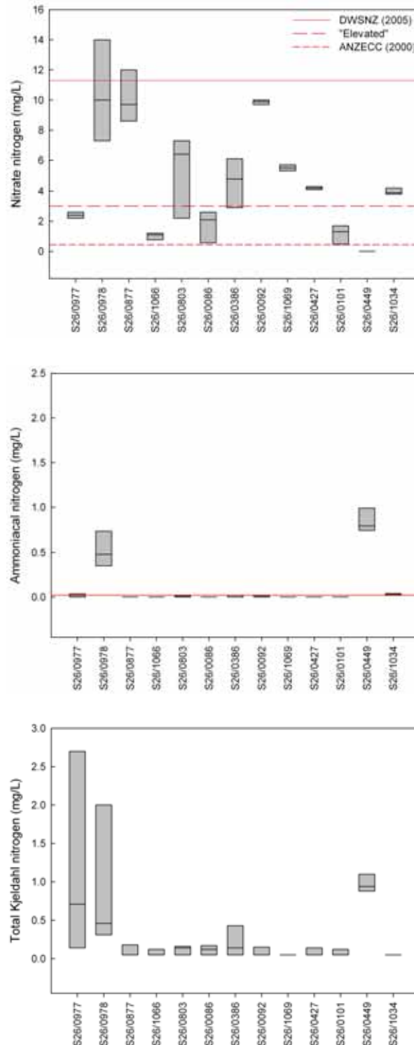
Figure 5.4: Box-and-whisker plots of nitrate-nitrogen, ammoniacal nitrogen and TKN concentrations in groundwater samples collected from 13 bores in the Mangatarere catchment at two-monthly intervals over October 2008 to October 2009 ( n=7 ). The three lines indicate in the first plot represent the DWSNZ (2005) MA, the "elevated" nitrate nitrogen threshold and the ANZECC (2000) trigger value for nitrite-nitrate nitrogen in lowland streams.
